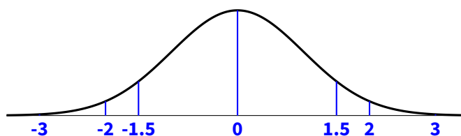
Figure 3: An illustration of how values that fall more than 2 or 3 SDs from the mean can be considered “in the tail” of the distribution
